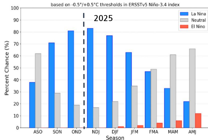
Figure 7. Official ENSO probabilities for the Niño 3.4 sea surface temperature index ( 5^{\circ}\text{N} - 5^{\circ}\text{S} , 120^{\circ}\text{W} - 170^{\circ}\text{W} ). Figure updated 12 September 2024.
