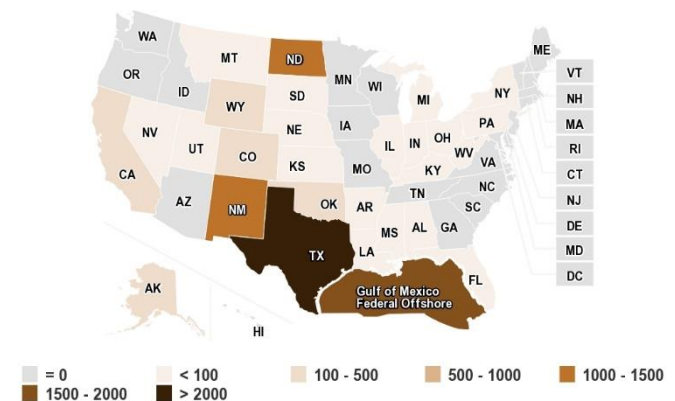
U.S. crude oil production by state in 2020 1,000 barrels per day
