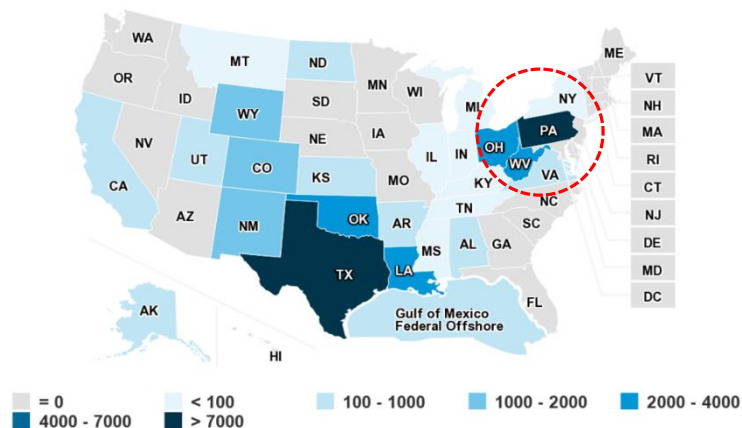
U.S. dry natural gas production by state in 2020 billion cubic feet
